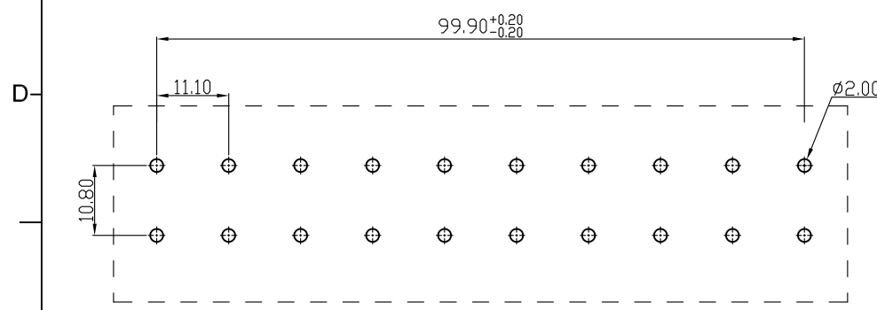
PCB LAYOUT
