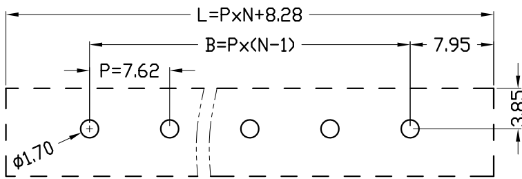
PCB LAYOUT
